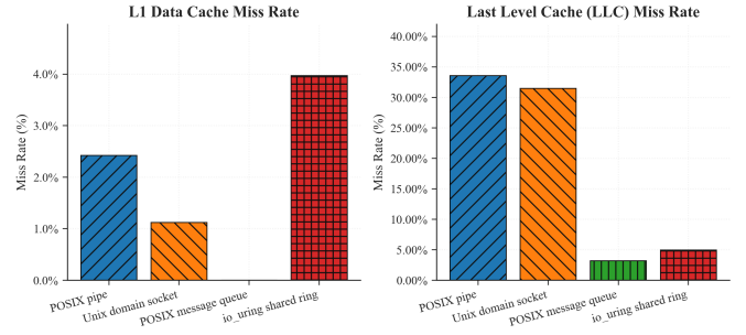
Fig. 9. L1 D-Cache and LLC Miss Rates by IPC Mechanism. Pipe and Socket exhibit \approx 30\text{--}34\% LLC miss rates due to kernel buffer staging evicting ring cache lines. SHM Ring (4.97 %) and POSIX MQ (3.2 %) achieve low LLC miss rates by keeping data in the shared 18 MiB L3.
